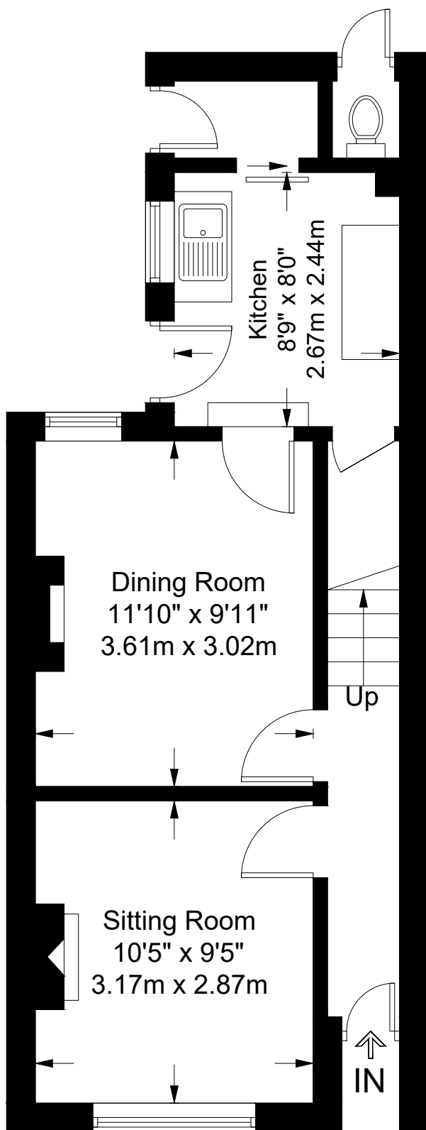
GROUND FLOOR
